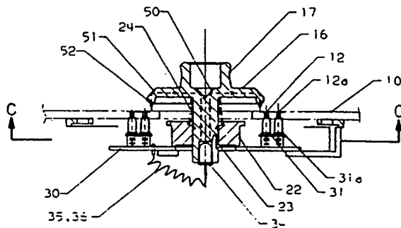
SECTION A-A - FIG 3
